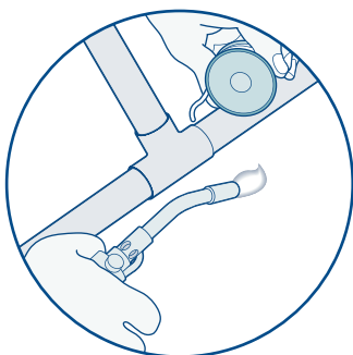
9(c). For end-feed fitting add limited solder after heating.
