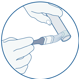
8(a). Applying flux to the outside of the tube
